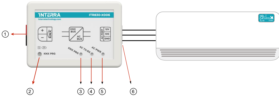
Fig. 3: Diagram of LG/Beko/Arcelik AC - KNX Gateway
