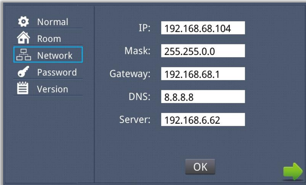
Fig. 33 : Network interface of the Indoor Panel
