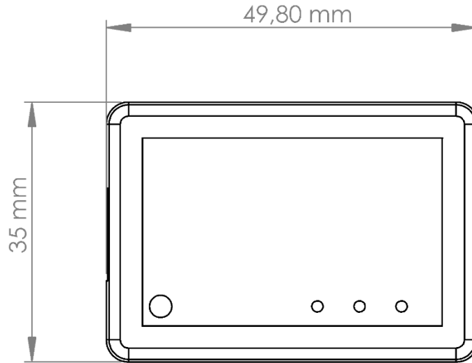
Fig. 1: Dimensions of Toshiba Split AC - KNX Gateway from the top view
