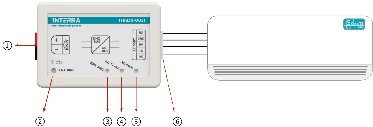
Fig. 3: Diagram of Toshiba Split AC - KNX Gateway
