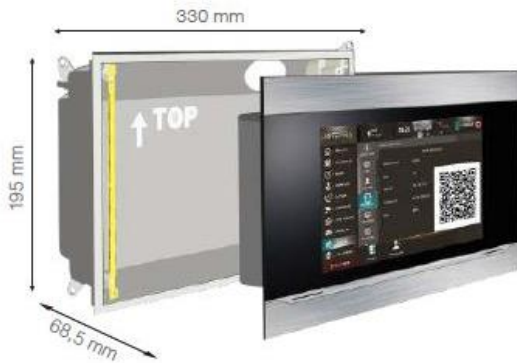
Interra 10,1" flush mounted receptacle I4 ITR-110-9004
