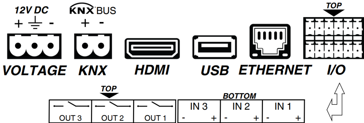
Fig. 3: Connectors
