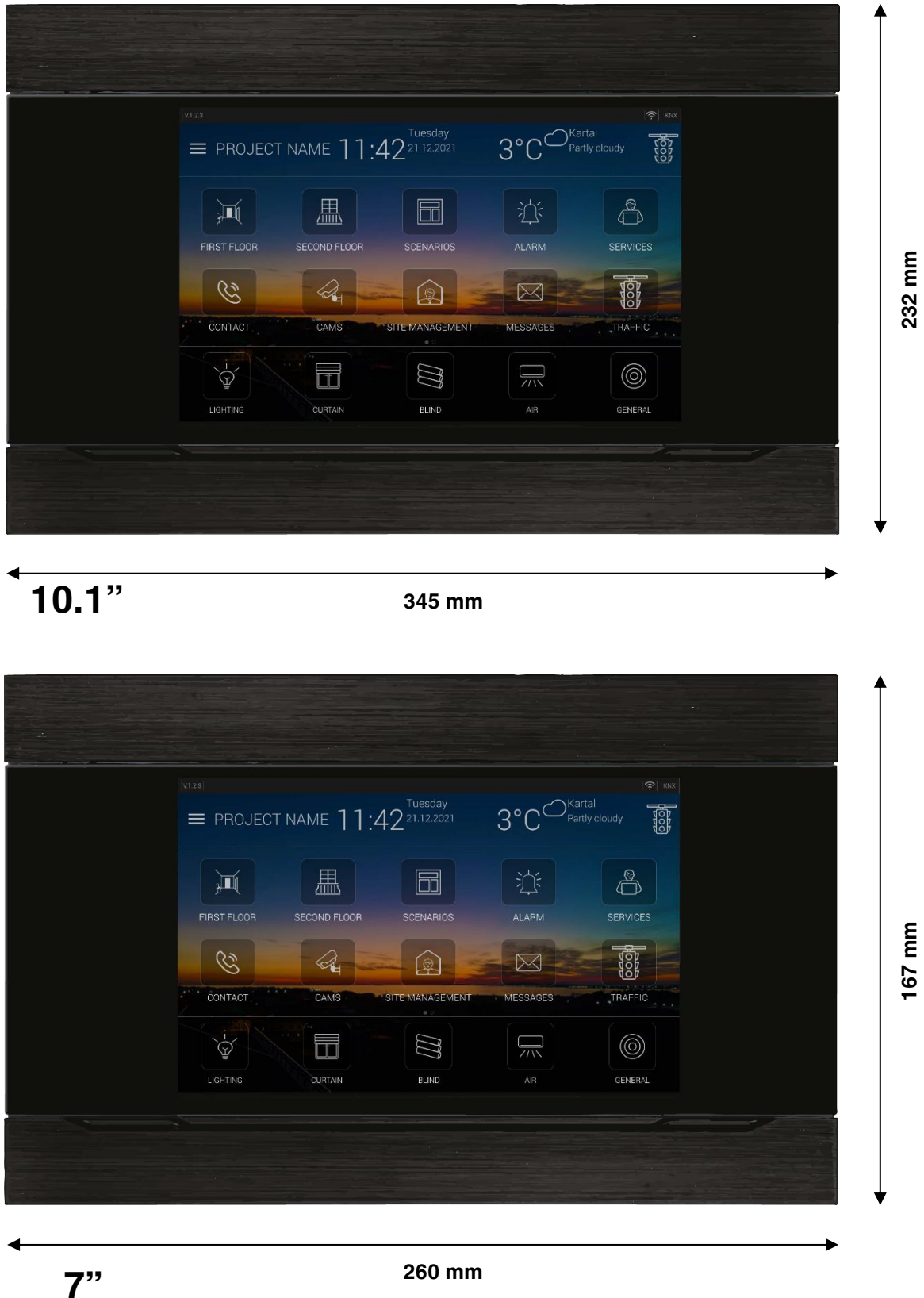
Fig. 1: Dimensions of all described device types
