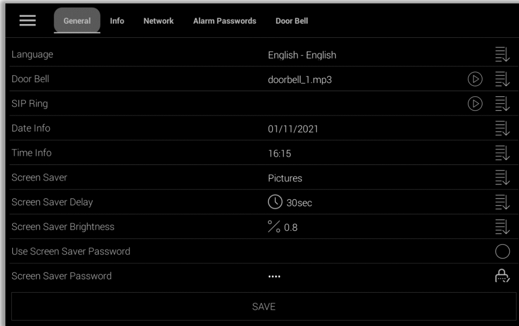
Fig. 50: Settings General
