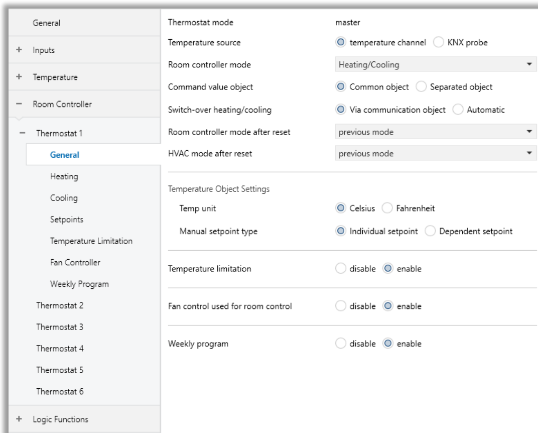
Fig. 20: Room Controller Thermostat General Configuration Page
