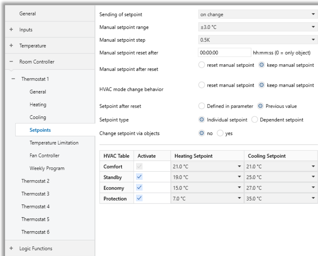
Fig. 34: Set Points Configuration Page
