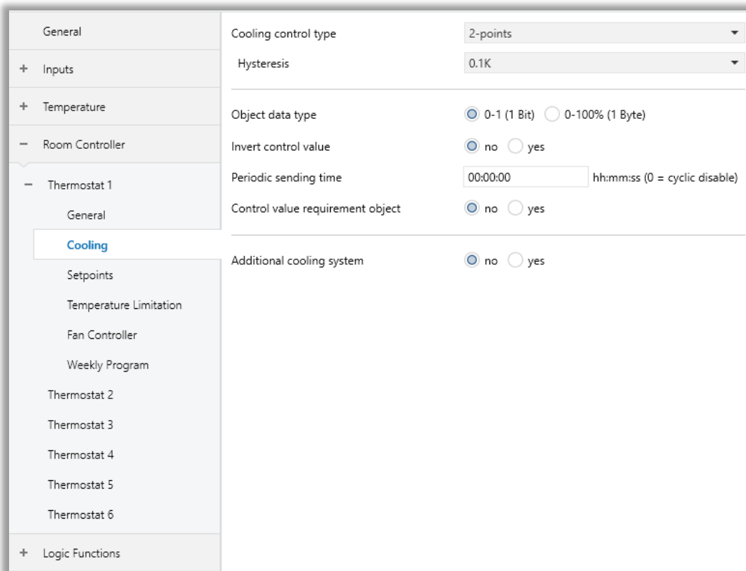
Fig. 27: Cooling 2-Points Control Configuration Page
