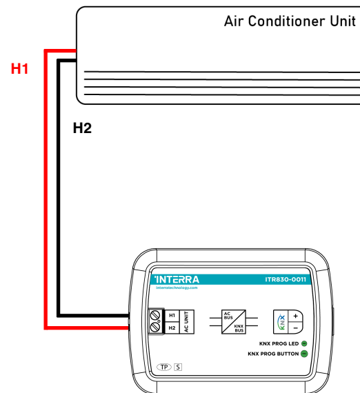
Demirdokum AC - KNX Gateway — Single Indoor Unit :
