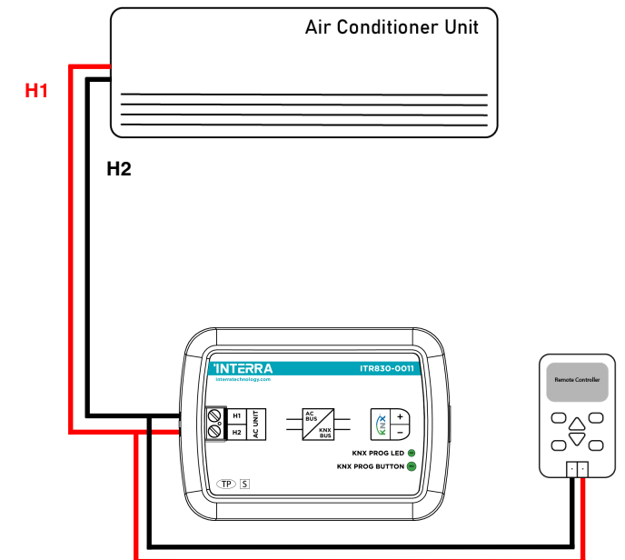
Demirdokum AC - KNX Gateway — Single Indoor Unit + Remote Controller :
