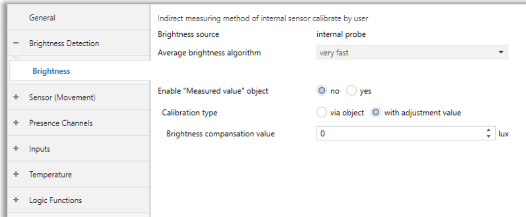
Fig. 14: Brightness Configuration Page
