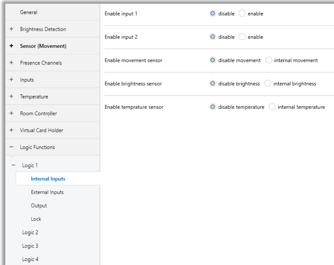
Fig. 67: Logic Functions – Input Configuration Page
