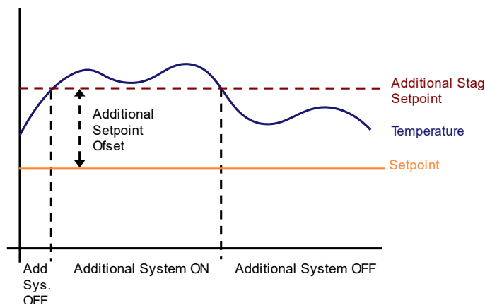
Fig. 52: PI Continuous Graph for Additional Cooling Control
