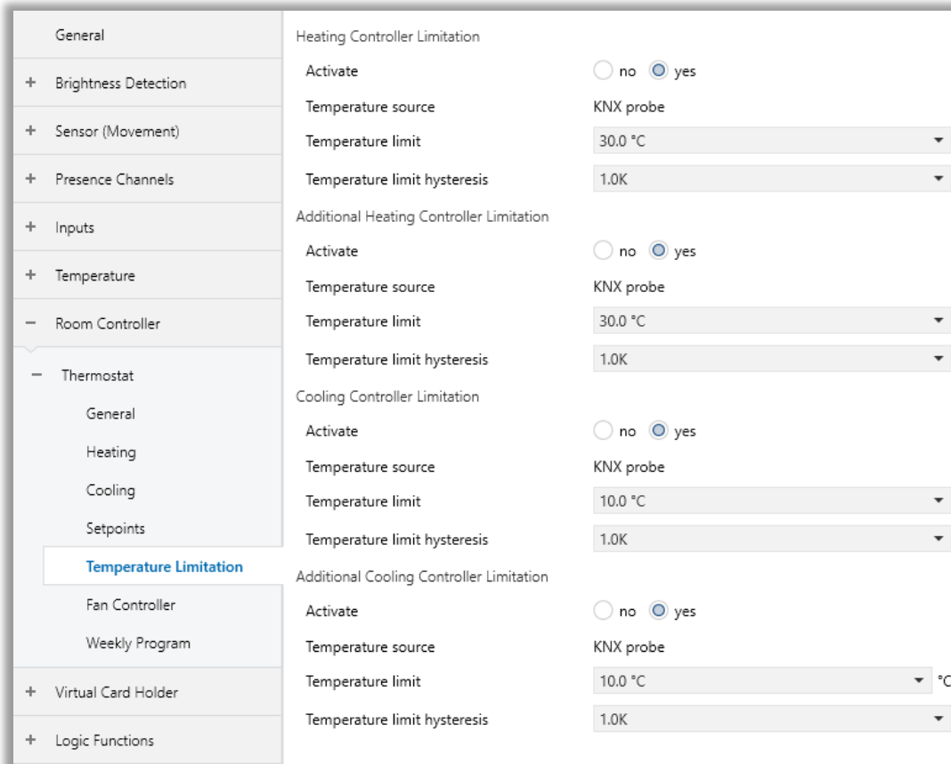
Fig. 55: Temperature Limitation Configuration Page
