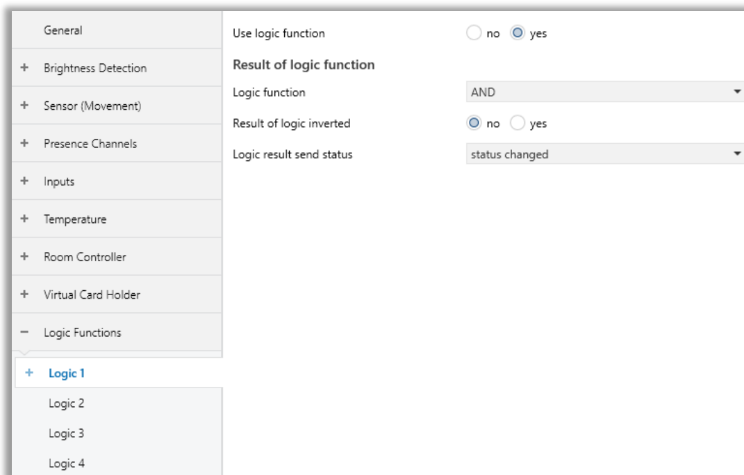
Fig. 66: Logic Functions – General Configuration Page
