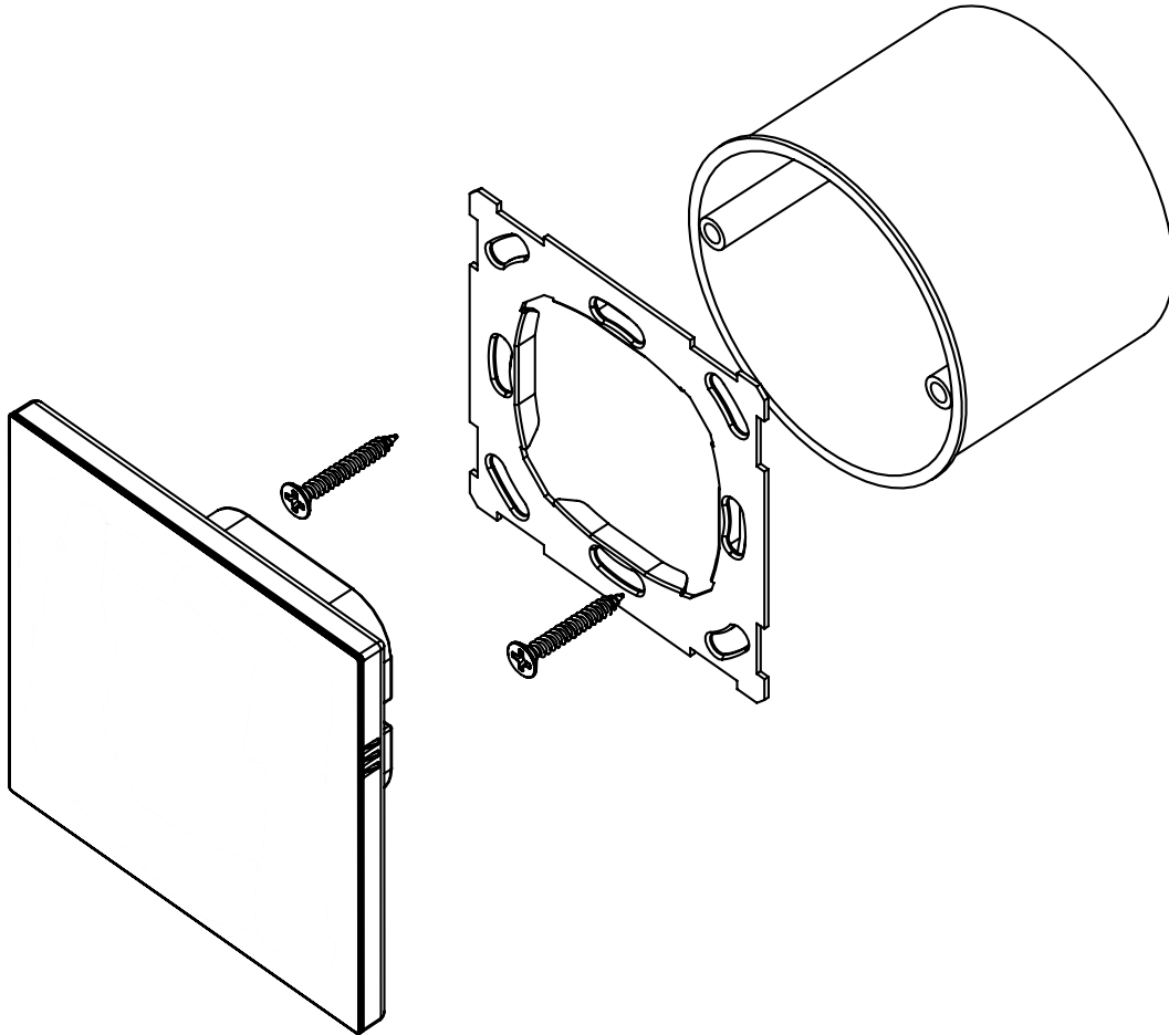
Fig. 6: Mounting the to Flush Mounting Box
