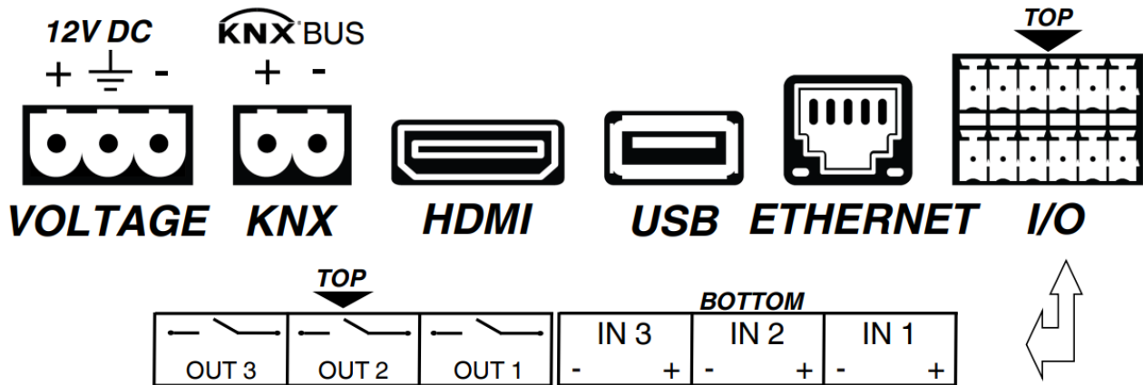
Fig. 3: Connectors
