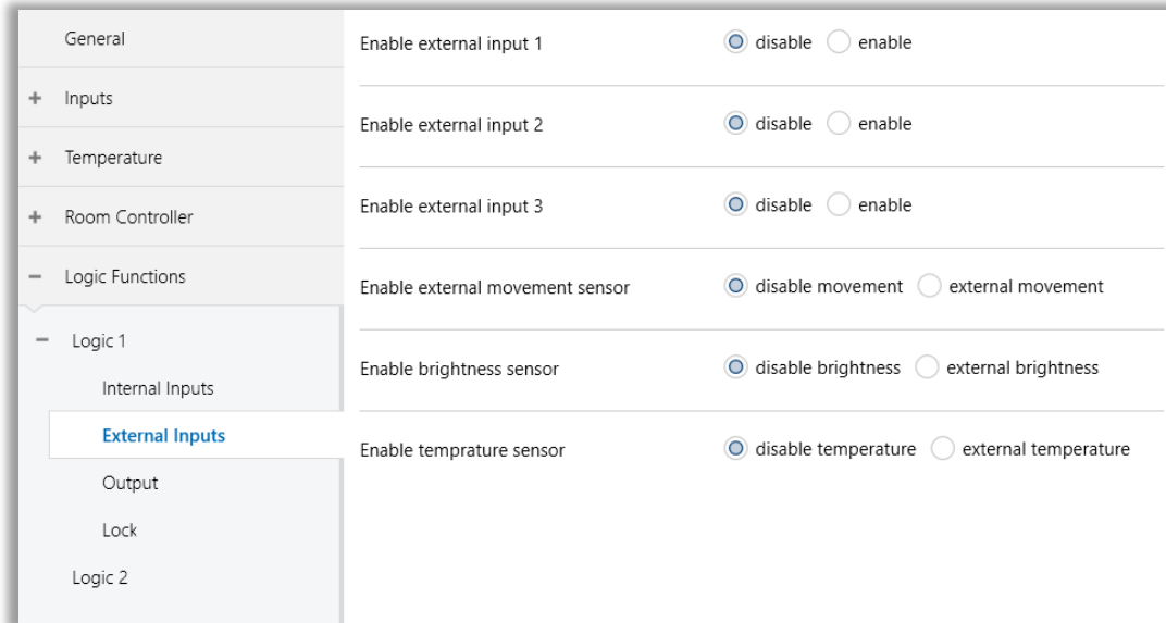
Fig. 30: Logic Functions – External Input Configuration Page
