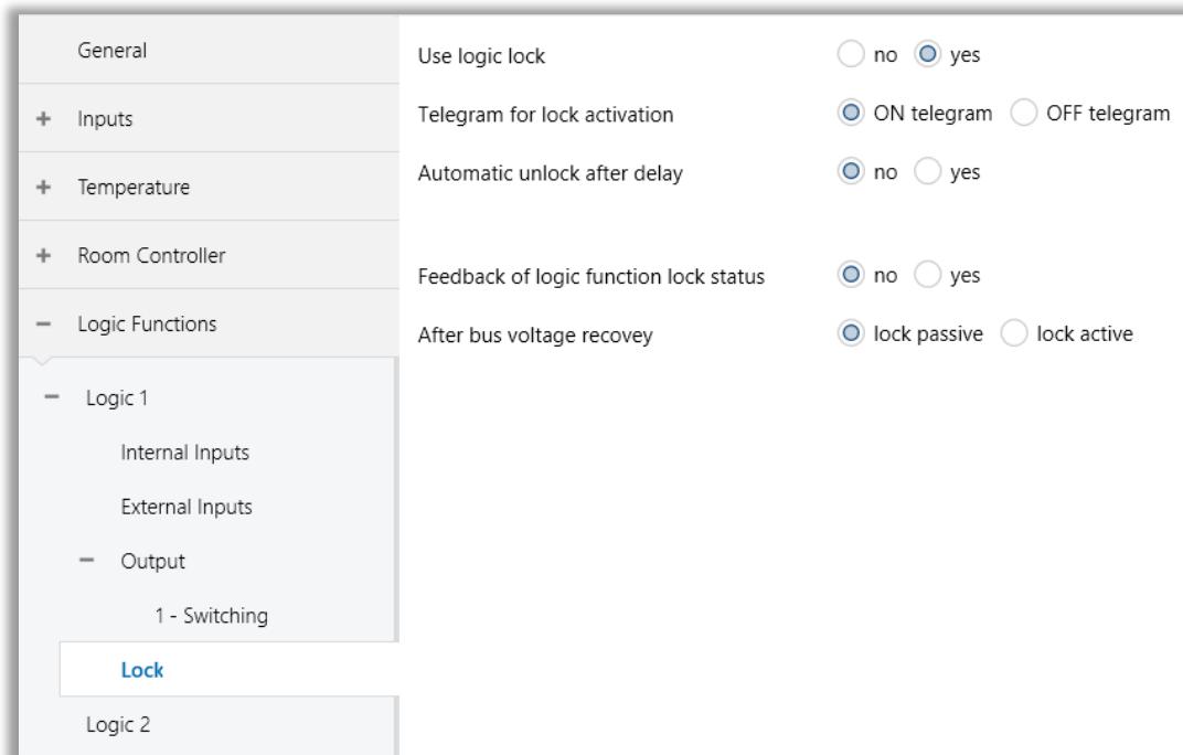
Fig. 33: Logic Functions – Lock Configuration Page
