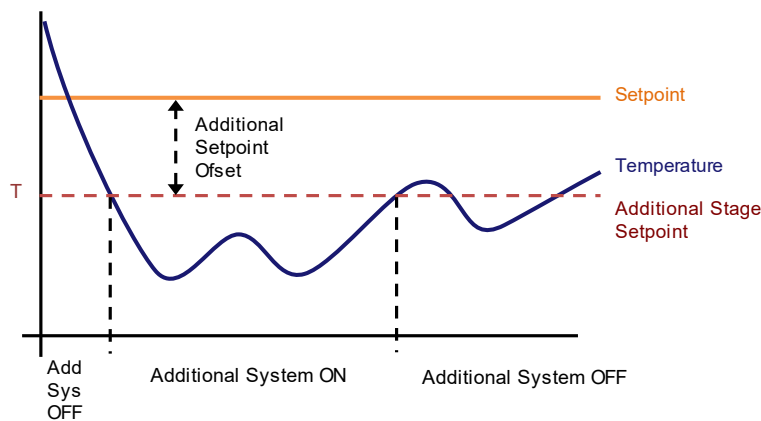
Fig. 25: 2 – Points Hysteresis Cycle for Additional Heating Control
