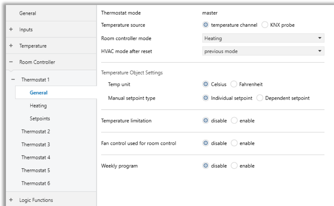
Fig.20: Thermostat General Configuration Page
