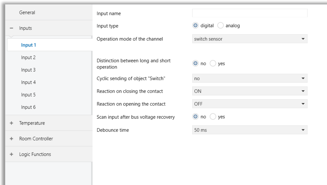
Fig. 4: Input – Switch Sensor Configuration Page
