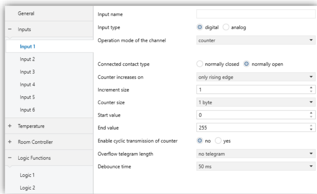
Fig. 12: Input – Counter Configuration Page
