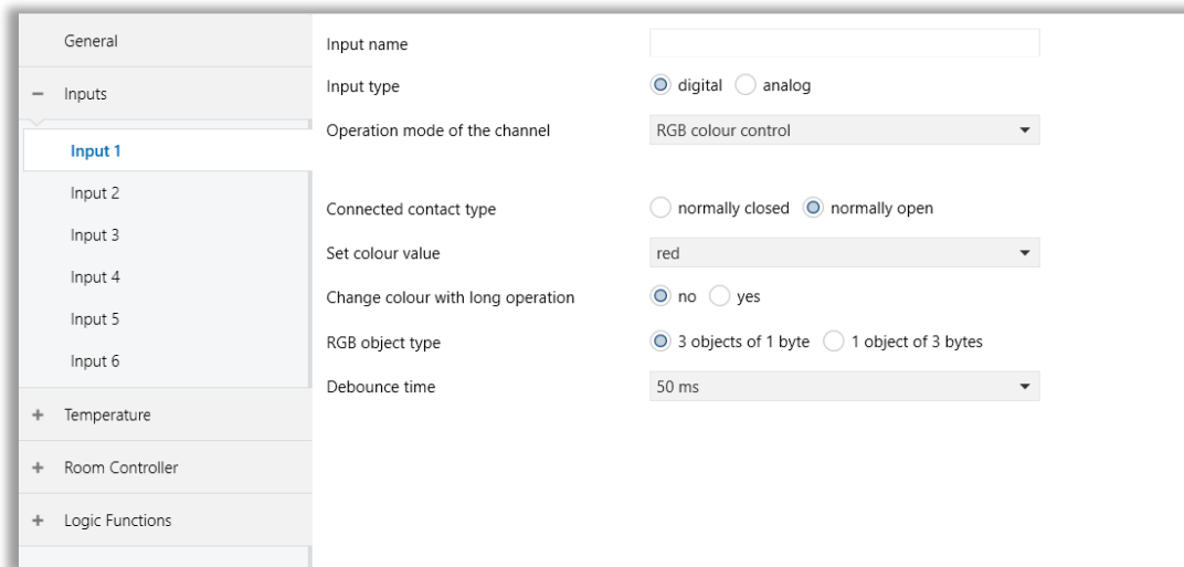
Fig. 9: Input – RGB Colour Control Configuration Page
