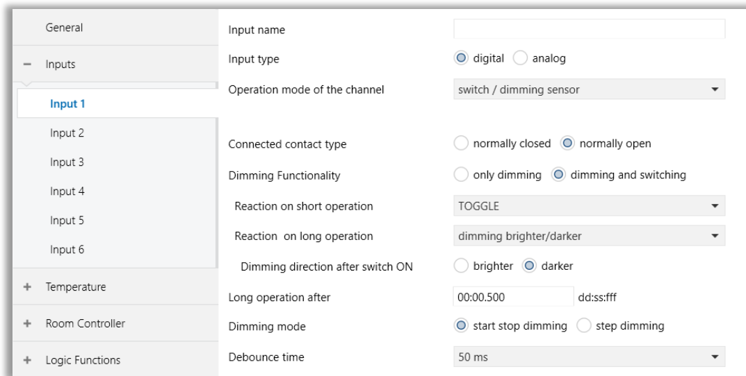
Fig. 5: Input – Switch / Dimming Sensor Configuration Page
