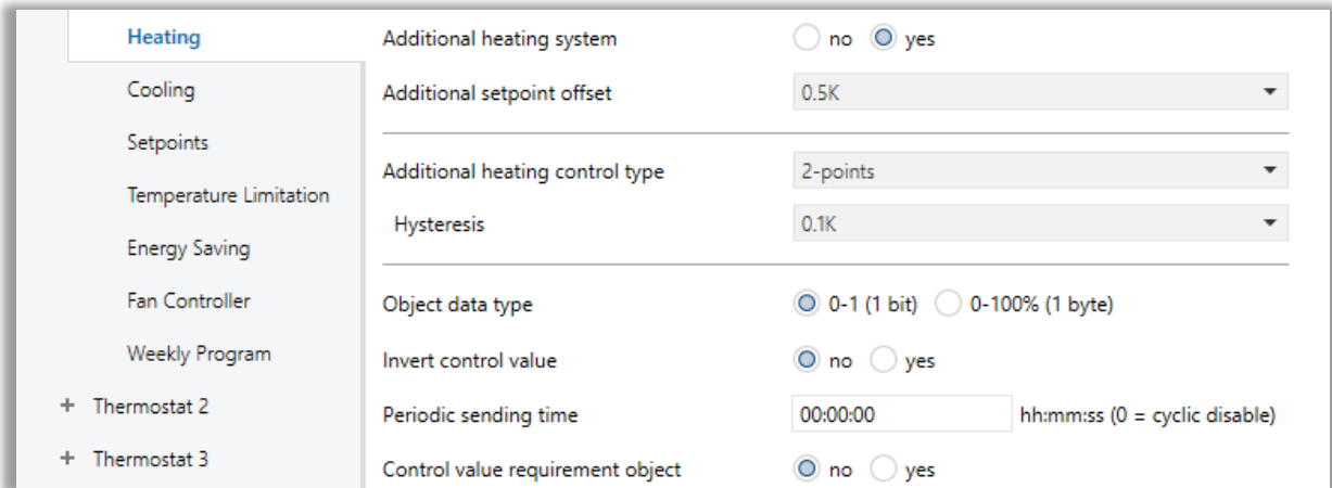
Fig. 48: Additional Heating System Configuration Page
