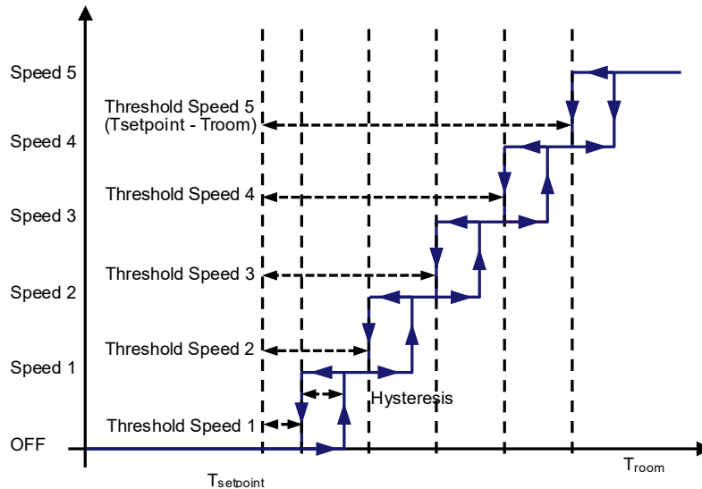
Fig. 63: Fan Controller 2-Points Control Cycle for Cooling
