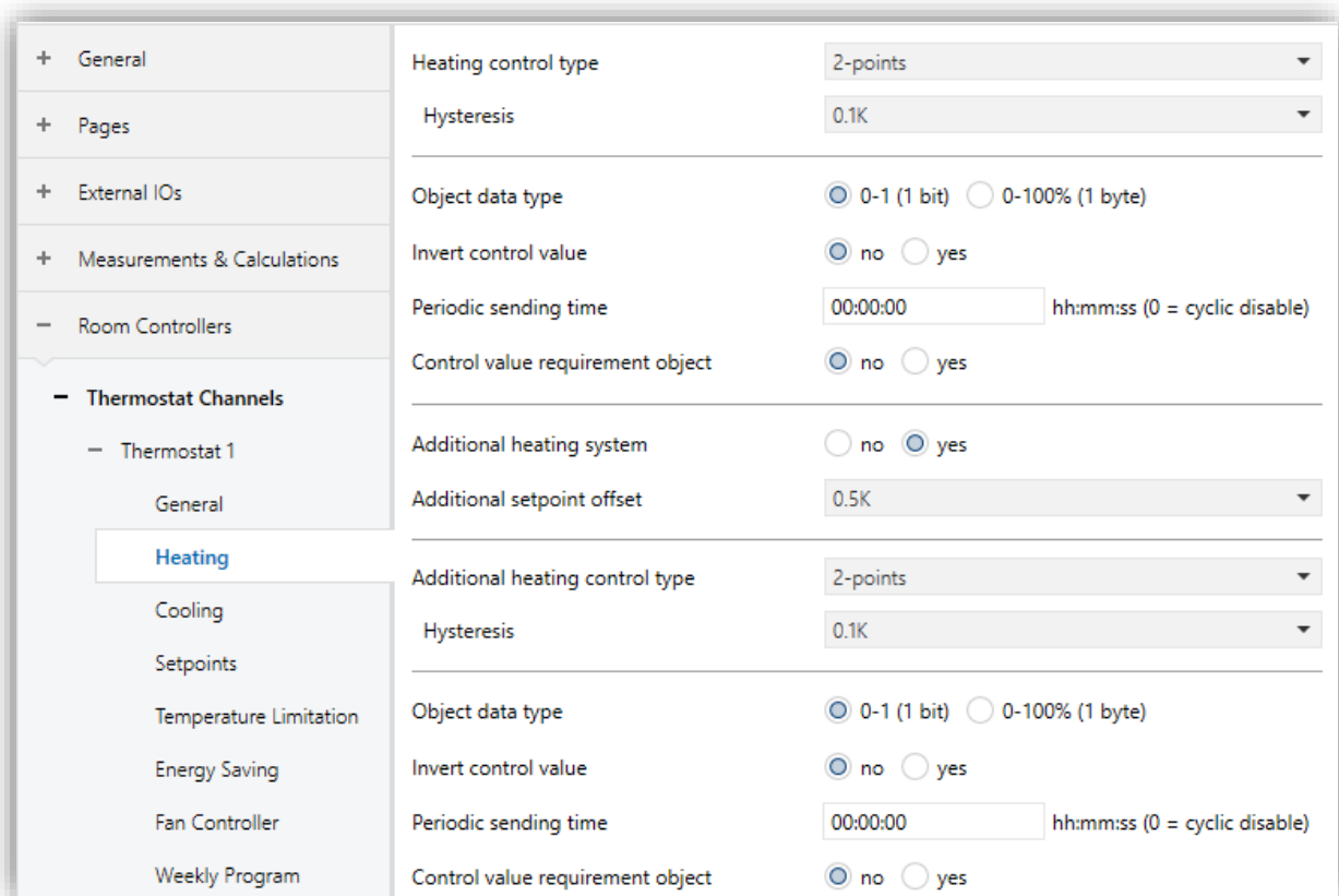
Fig. 45: Heating 2-Points Control Configuration Page
