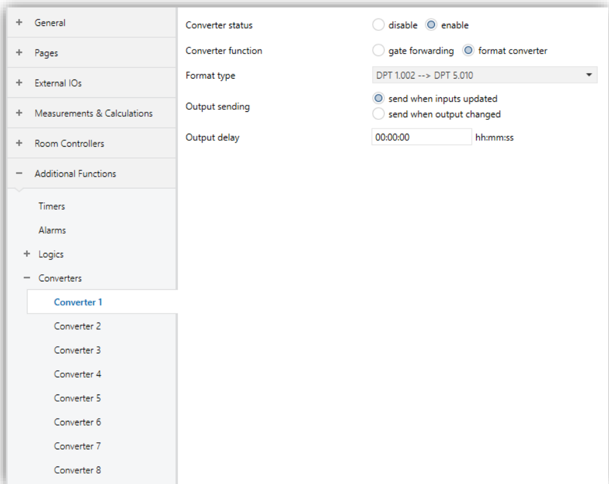
Fig. 82: Logics – Format Converter Configuration Page
