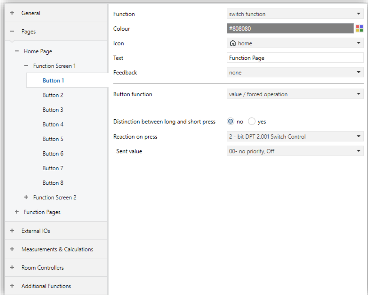
Fig. 15: Value/Forced Operation Function Configuration Page
