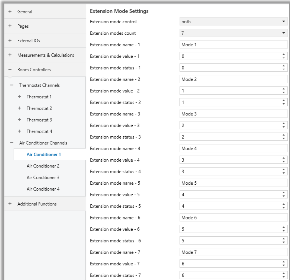
Fig. 69: Air Conditioner – Extension Mode Settings Configuration Pages
