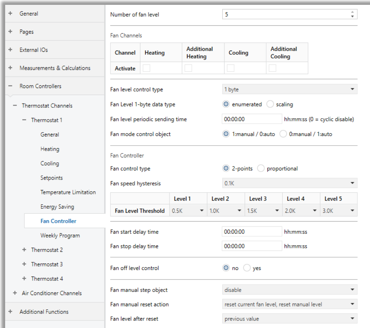
Fig. 61: Fan Controller 2-Points Control Configuration Page
