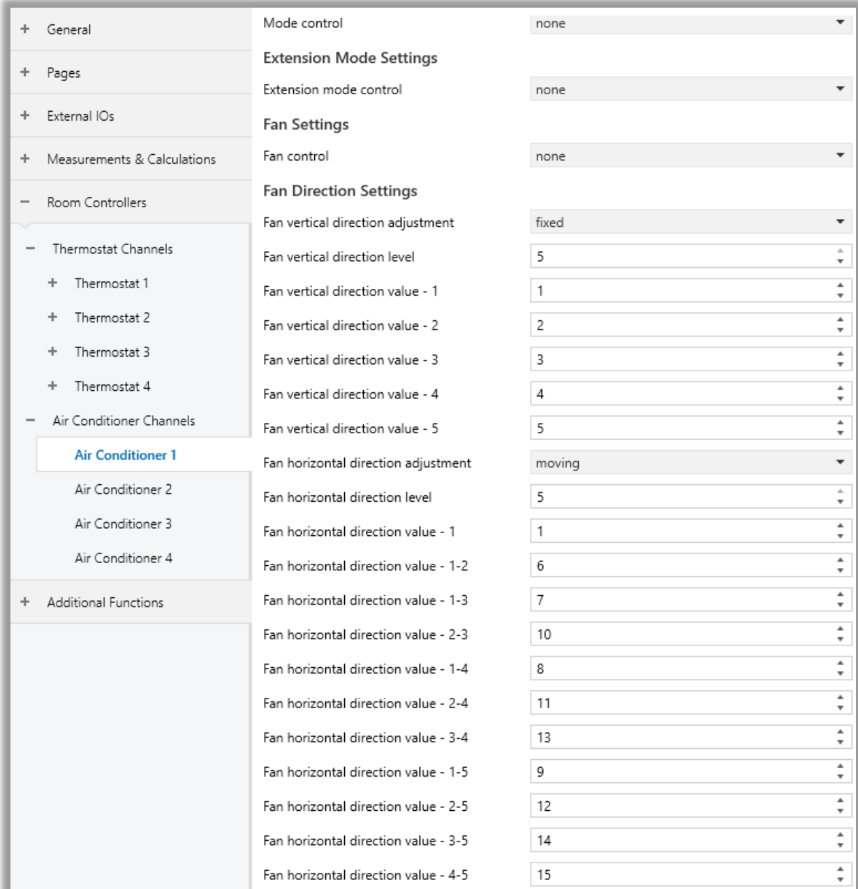
Fig. 71: Air Conditioner – Fan Direction Settings Configuration Page
