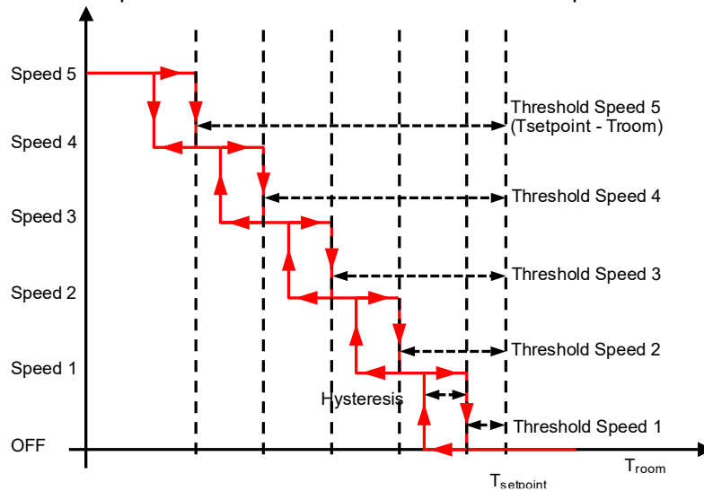
Fig. 62: Fan Controller 2-Points Control Cycle for Heating
