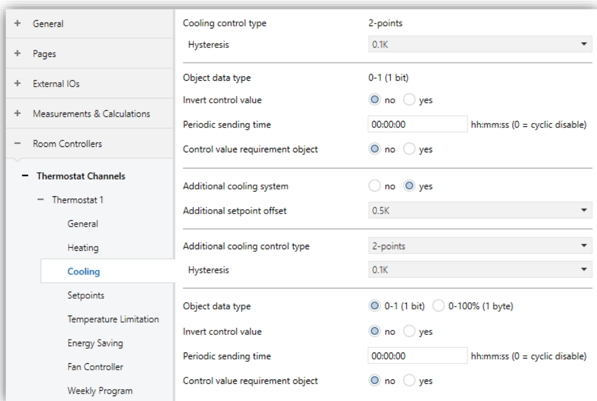
Fig. 51: Cooling 2-Points Control Configuration Page
