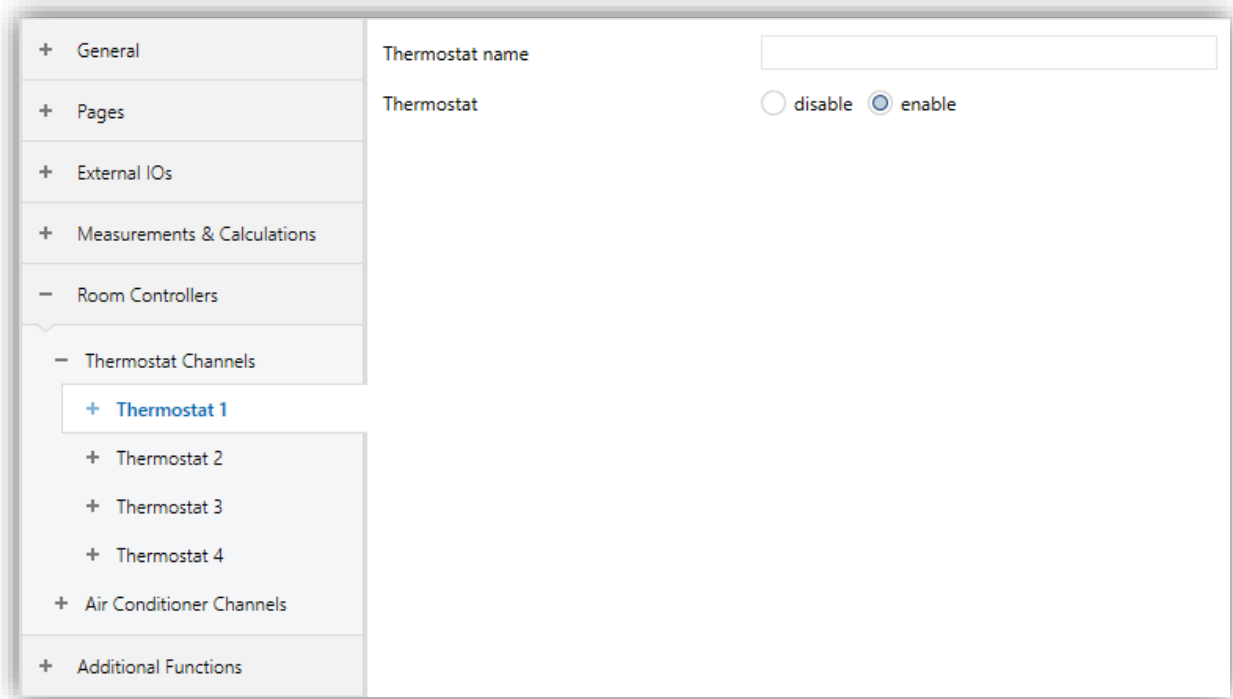
Fig. 43: Room Controller Thermostat Configuration Page
