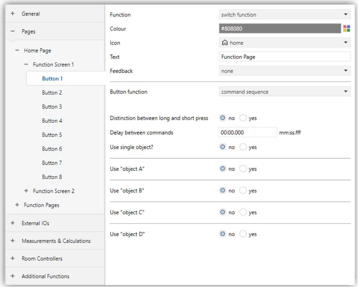
Fig. 18: Command Sequence Function Configuration Page
