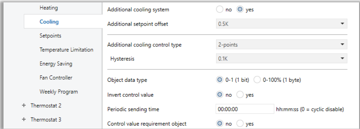
Fig. 54: Additional Cooling System Configuration Page
