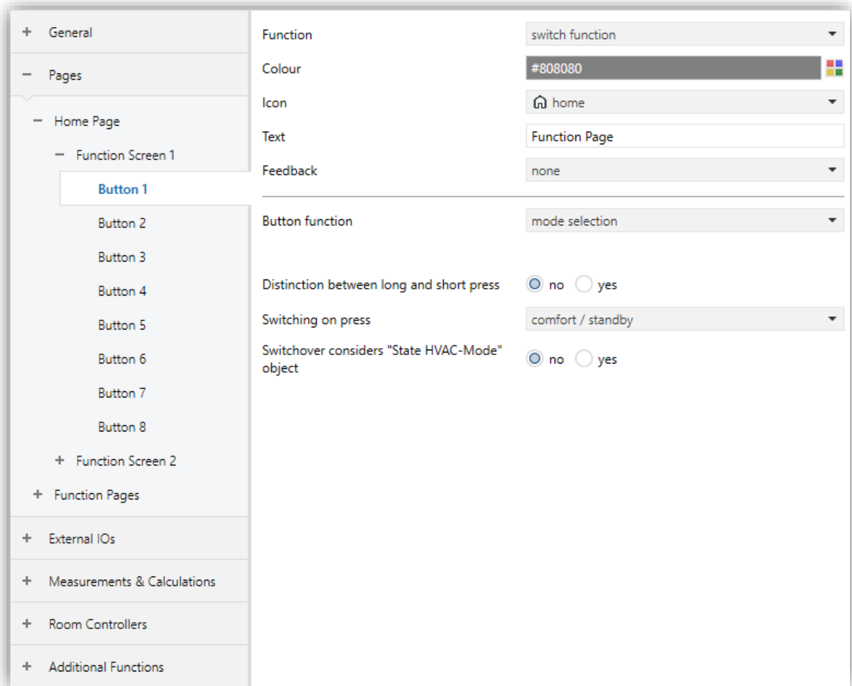
Fig. 17: Mode Selection Function Configuration Page
