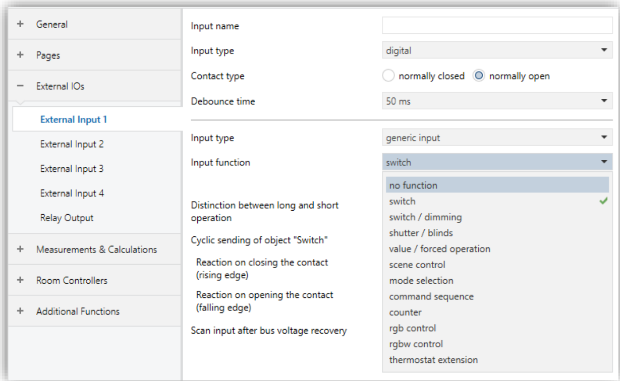
Fig. 28: Digital Input – Generic Input Page
