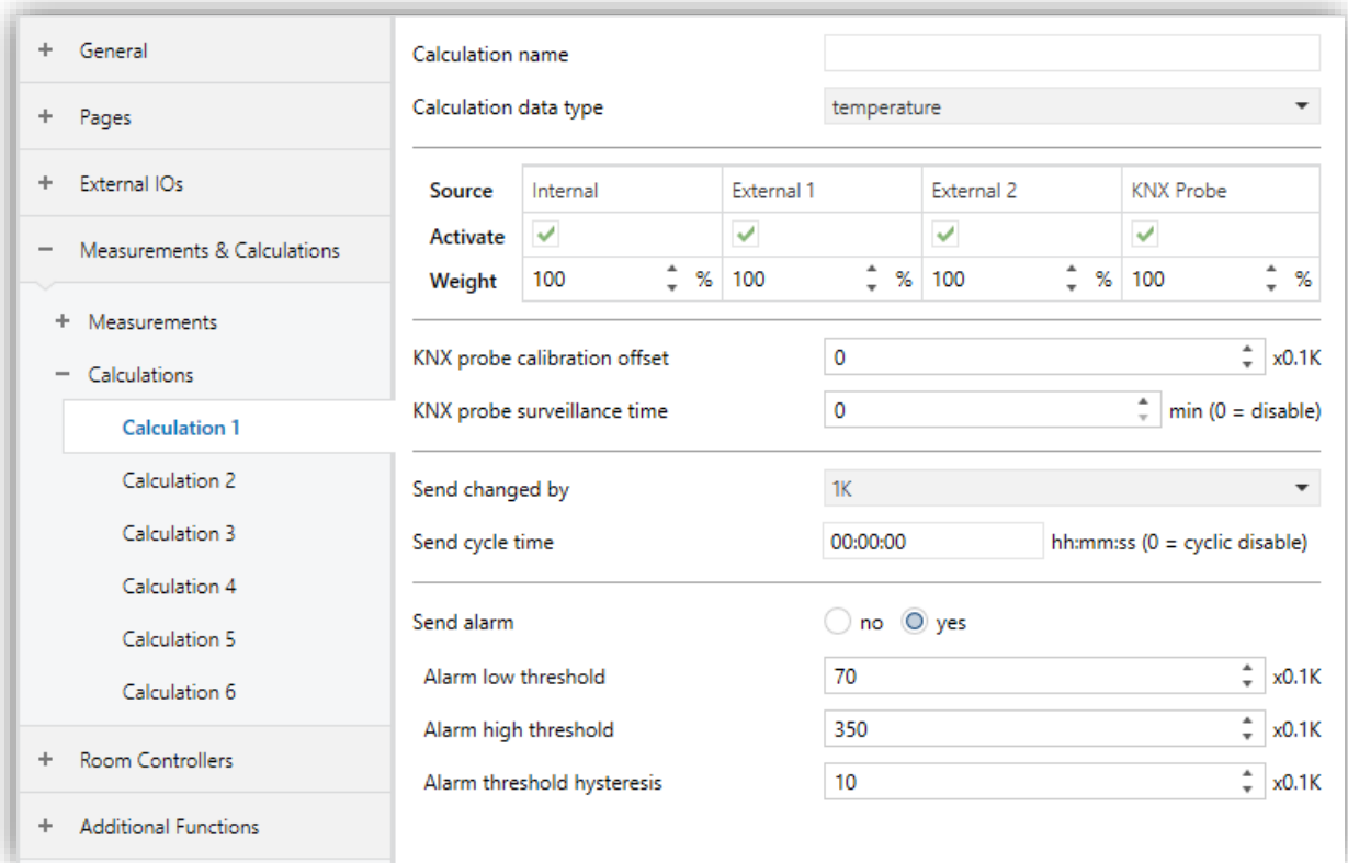
Fig. 39: Calculation for Temperature Page
