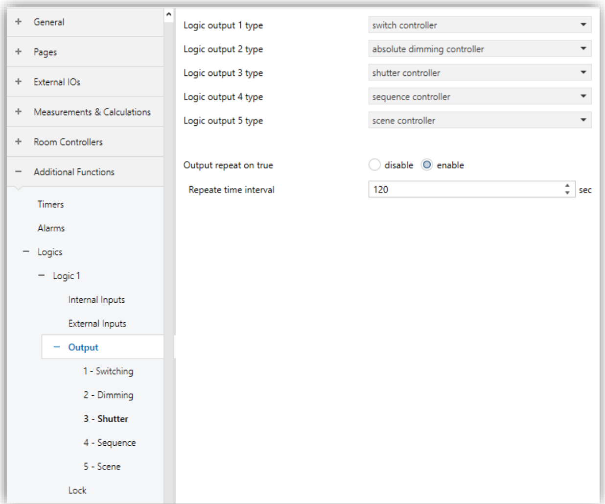
Fig. 79: Logics – Output 1-5 Configuration Page
