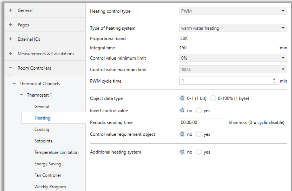
Fig. 46: Heating PWM Control Configuration Page
