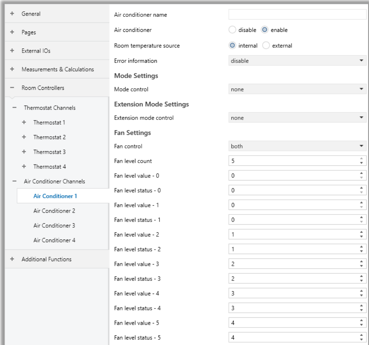
Fig. 70: Air Conditioner – Fan Settings Configuration Page
