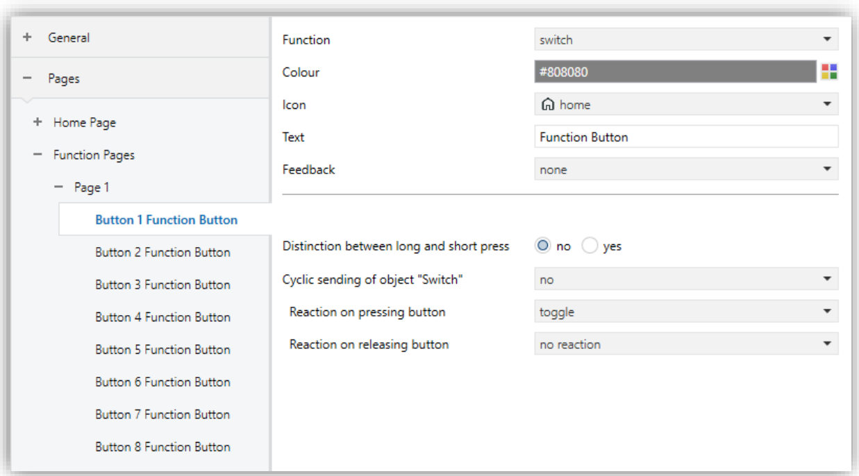
Fig. 11: Function Page - Button X Configuration Page
