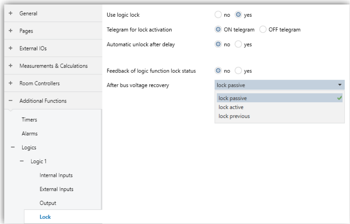
Fig. 80: Logics – Lock Configuration Page
