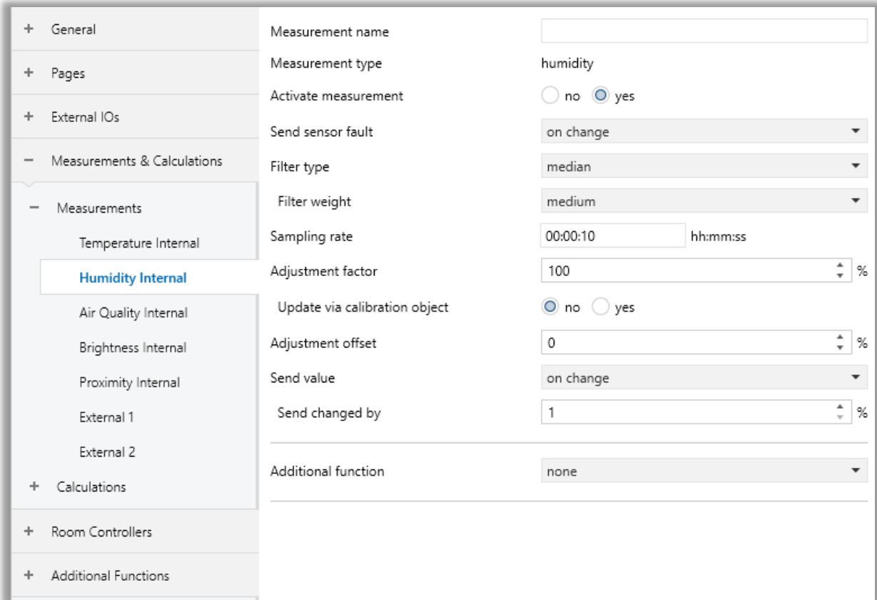
Fig. 32: Humidity Internal Page
