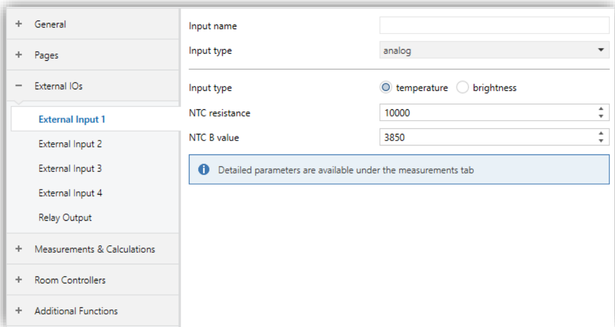
Fig. 26: Analog Input – Temperature Page
