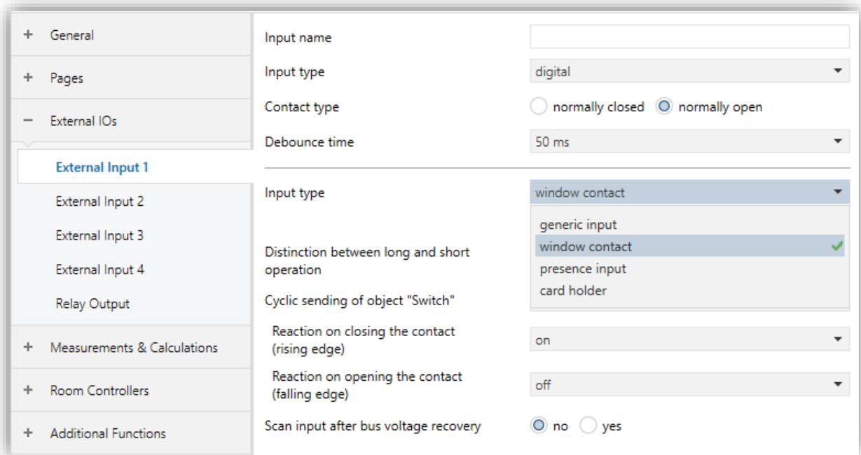
Fig. 29: Digital Input – Energy Saving Inputs
