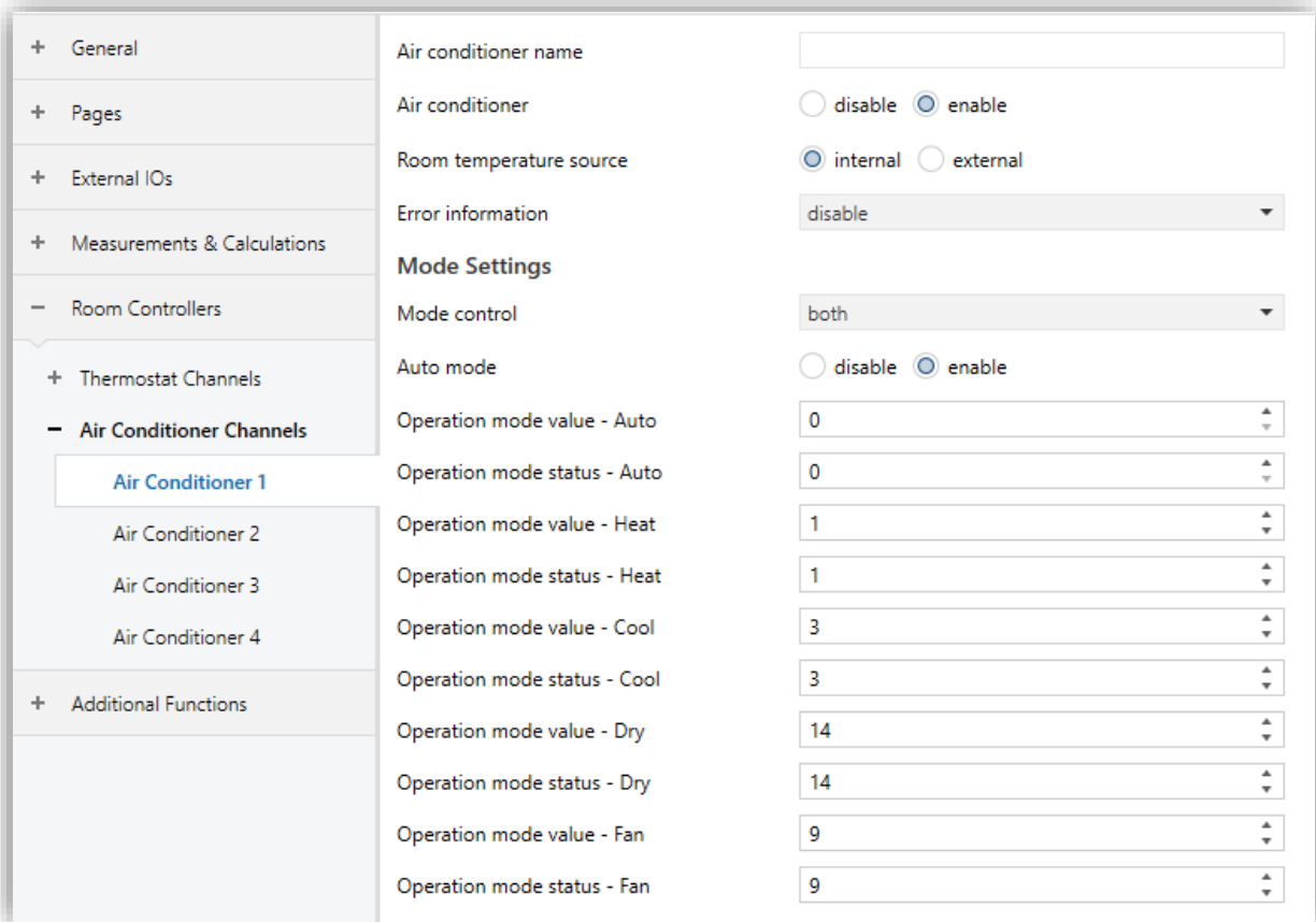
Fig. 68: Air Conditioner X – Mode Settings Configuration Page
