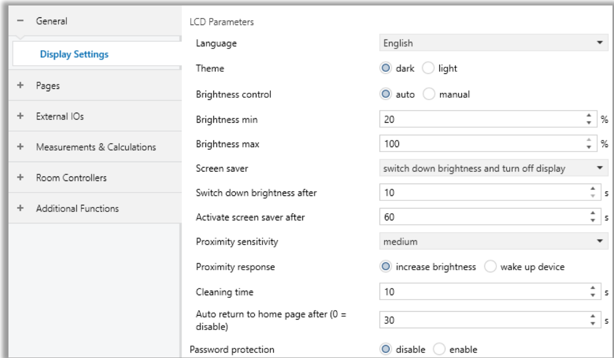
Fig. 5: Display Settings Configuration Page
