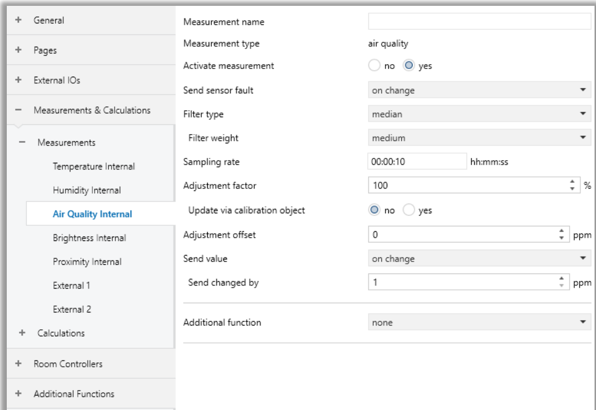
Fig. 33: Air Quality Internal Page
