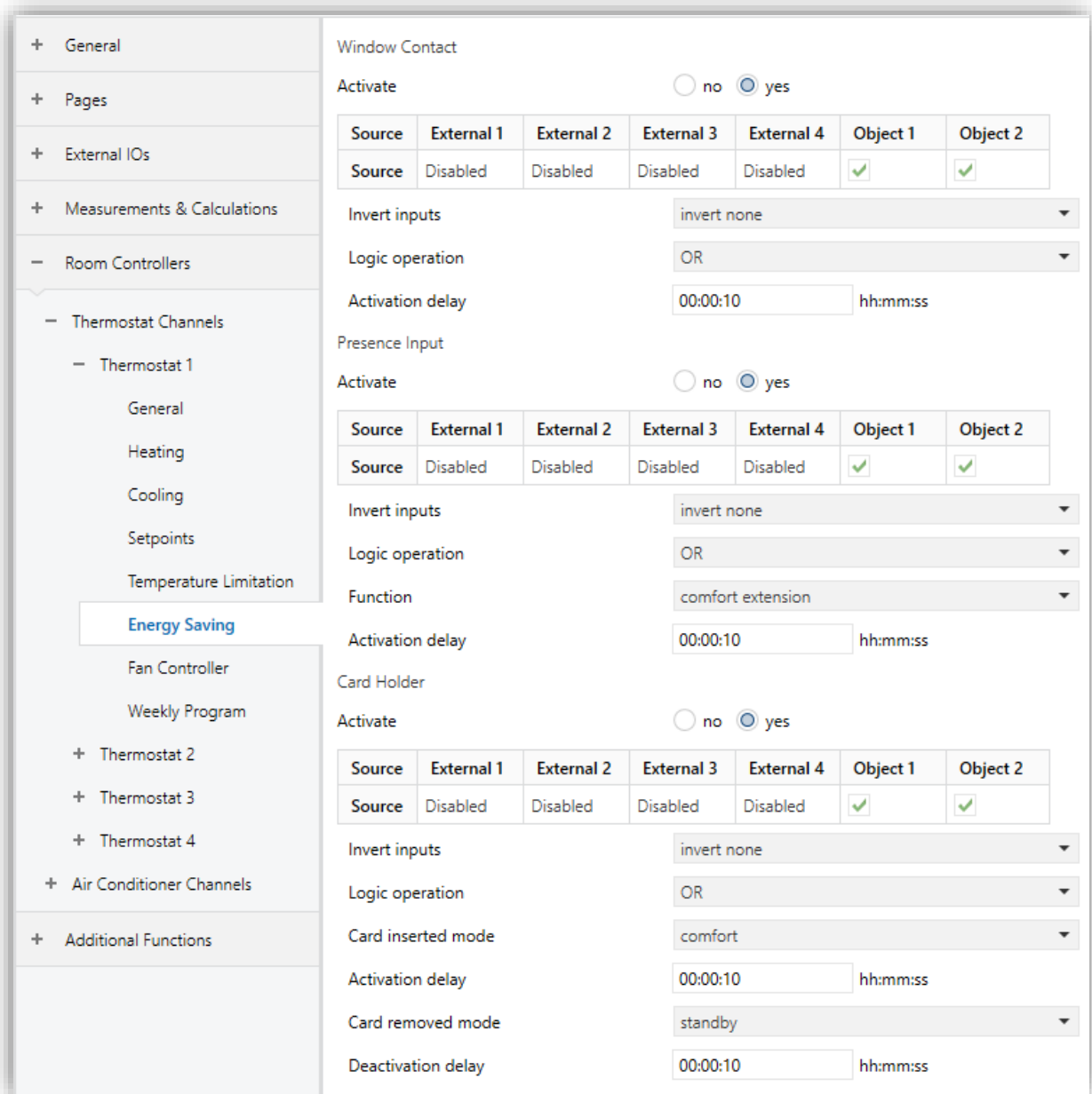
Fig. 60: Energy Saving Configuration Page
