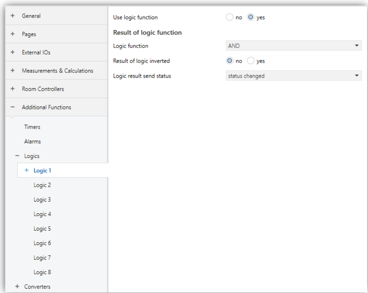
Fig. 75: Logics – General Configuration Page
