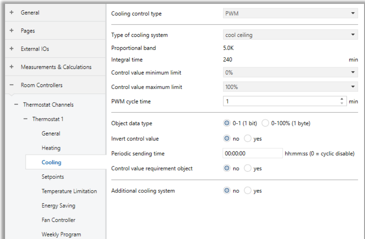
Fig. 52: Cooling PWM Control Configuration Page
