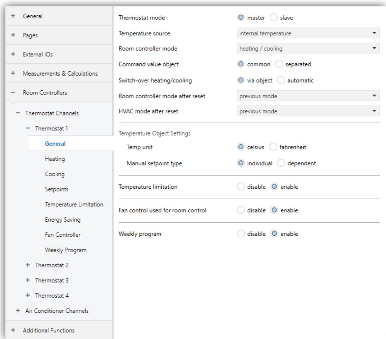
Fig. 44: Room Controller Thermostat General Configuration Page
