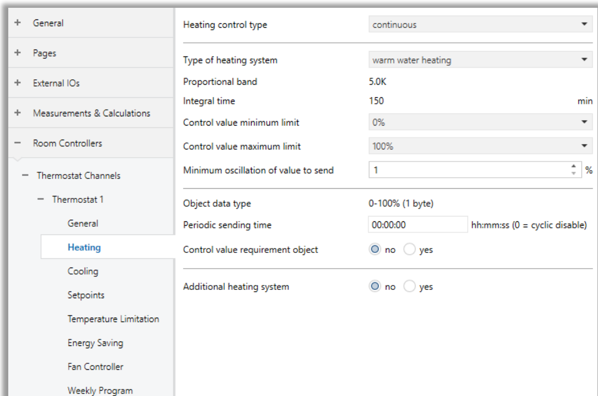
Fig. 47: Heating Continuous Control Configuration Page
