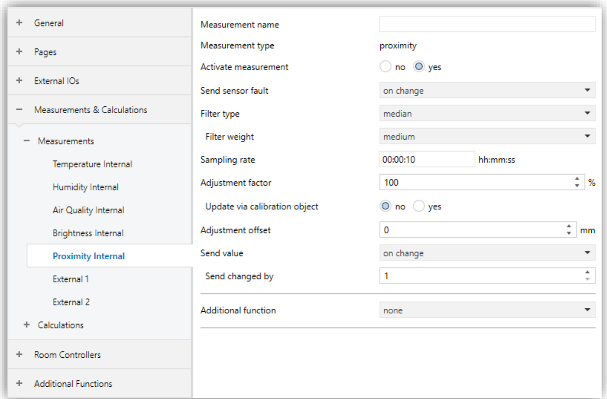
Fig. 36: Proximity Internal Page
