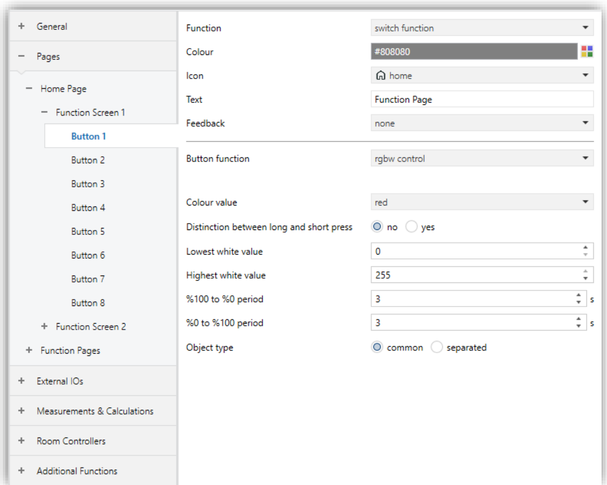
Fig. 21: RGBW Control Configuration Page
