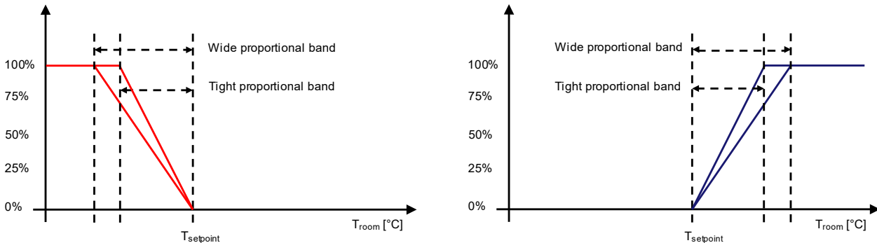
Fig. 36: Continuous PI Control Proportional Band Widths
