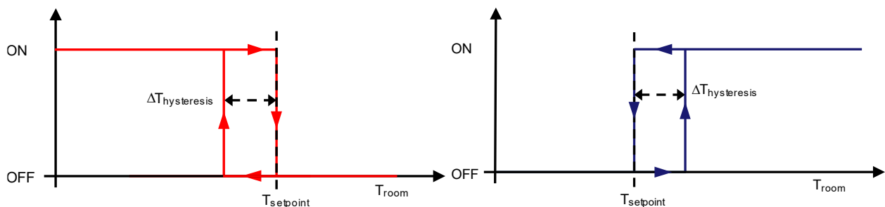
Fig. 35: 2 – Points Control Hysteresis Cycle
