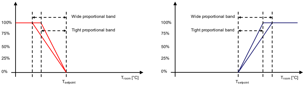
Fig. 59: Fan Controller Proportional Control
