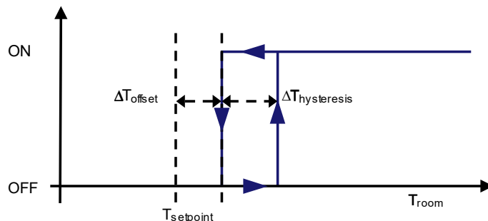
Fig. 50: 2 – Points Hysteresis Cycle for Additional Cooling Control
