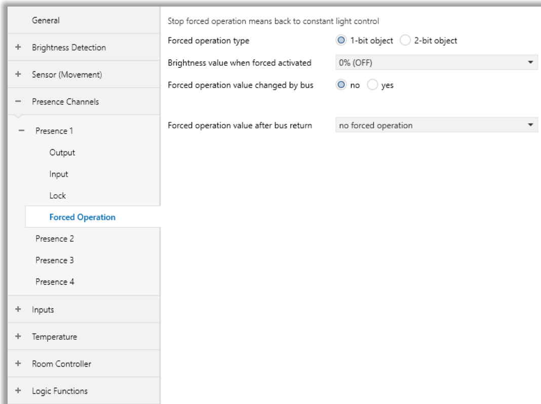
Fig. 21: Constant Light-Controller – Forced Operation Configuration Page
