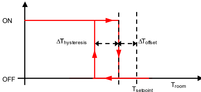
Fig. 44: 2 – Points Hysteresis Cycle for Additional Heating Control
