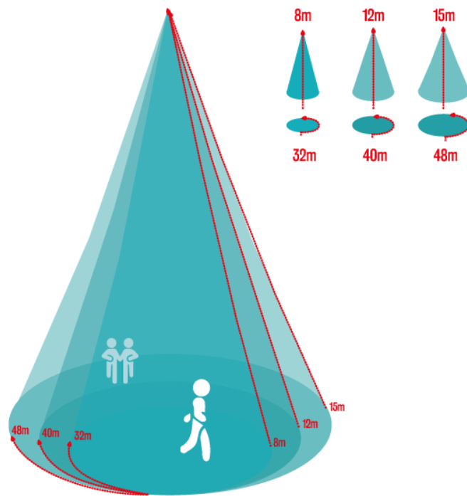
Fig. 5: High Bay Plus KNX Sensor Detection Range
