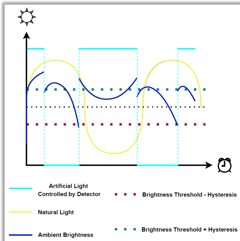
Fig. 10: Constant Light Switch Operation
