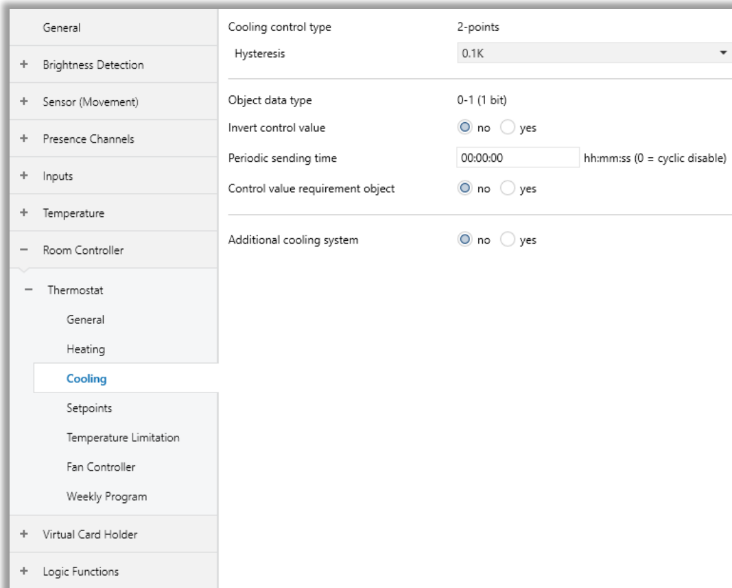
Fig. 46: Cooling 2-Points Control Configuration Page
