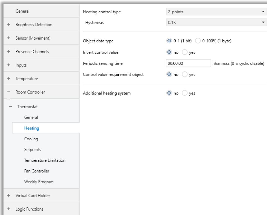
Fig. 40: Heating 2-Points Control Configuration Page
