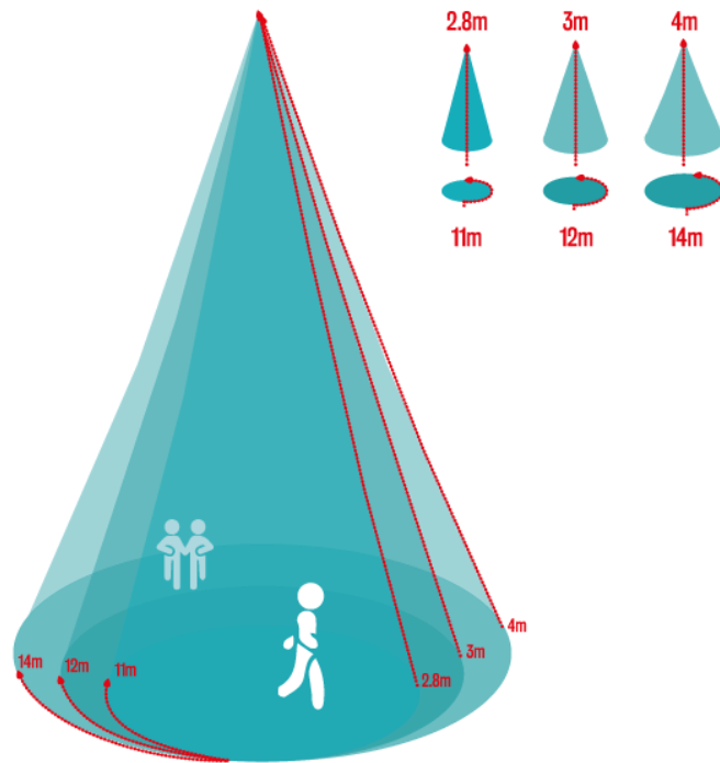
Fig. 6: Microwave KNX Sensor Detection Range
