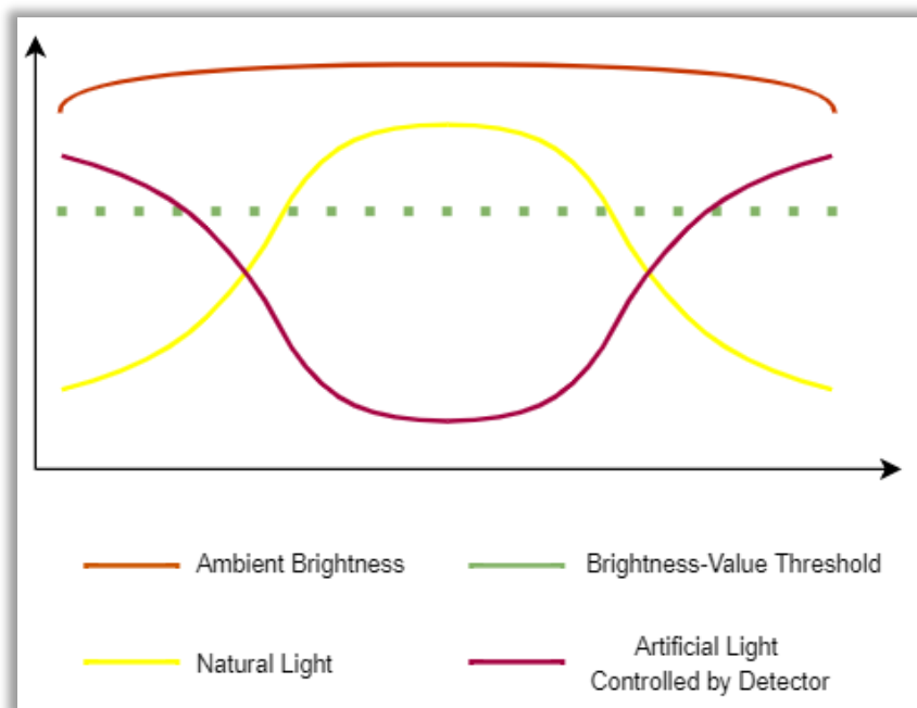
Fig. 11: Constant Light Control Operation
