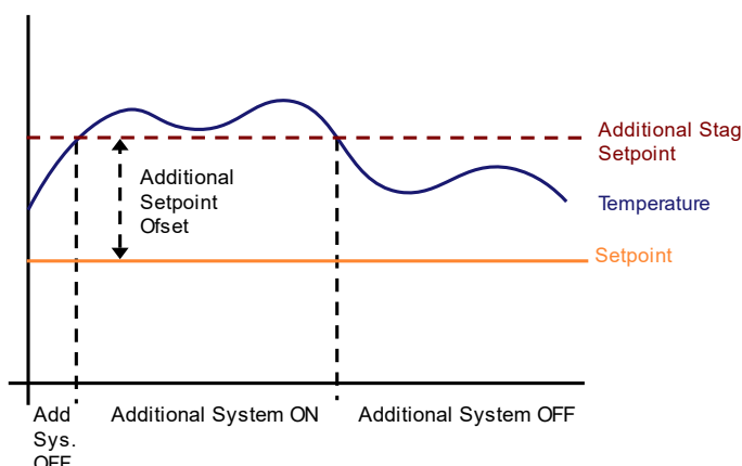
Fig. 51: PI Continuous Graph for Additional Cooling Control
