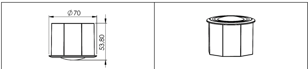
Fig. 9: Surface Mounted Dimensions Figure
