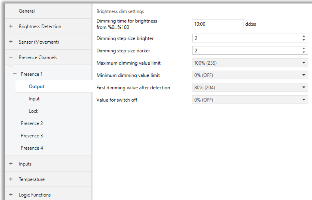
Fig. 18: Constant Light Controller - Output Configuration Page
