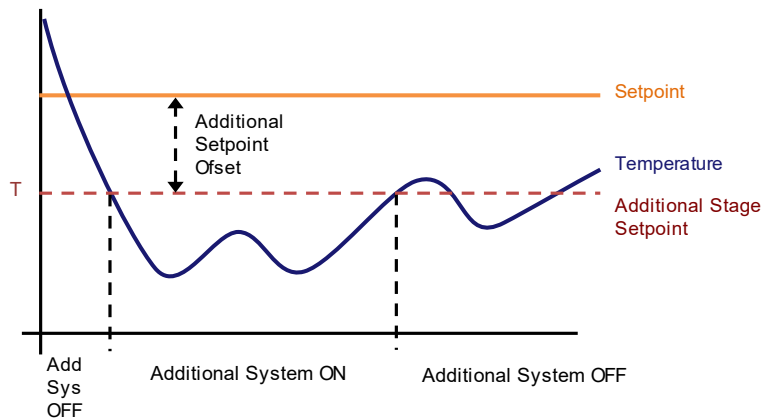
Fig. 45: PI Continuous Graph for Additional Heating Control
