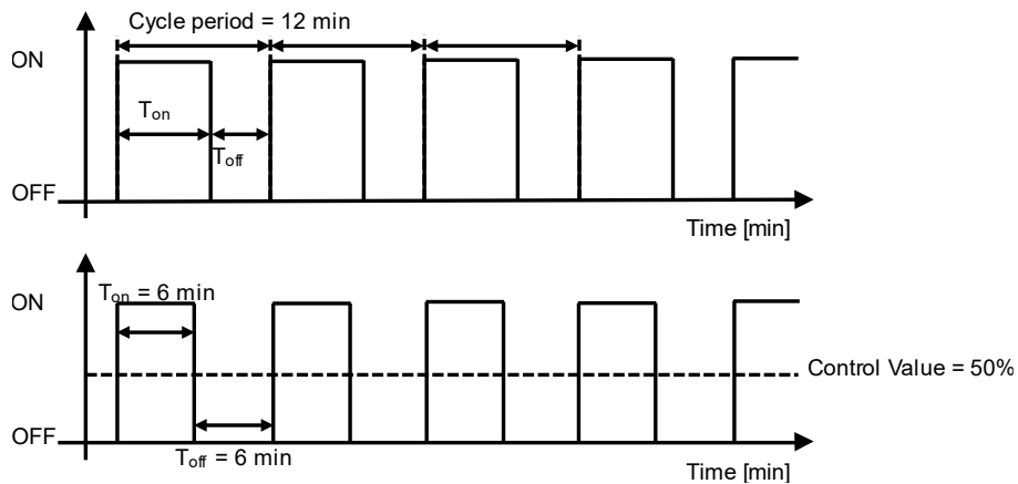
Fig. 37: PWM Control Sampling
