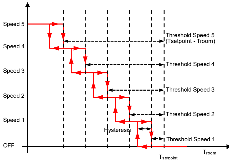
Fig. 56: Fan Controller 2-Points Control Cycle for Heating
