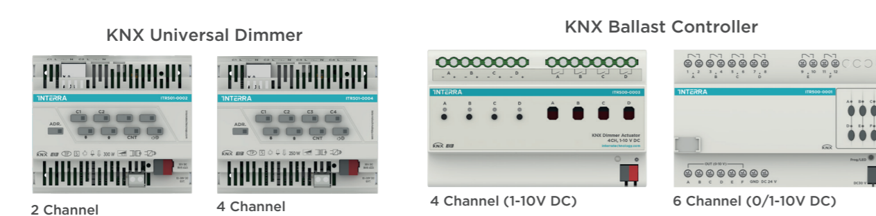
KNX Dimmer Actuators
