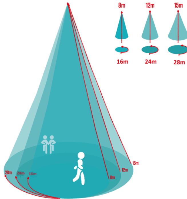
Fig. 4 : High Bay KNX Sensor Detection Range
