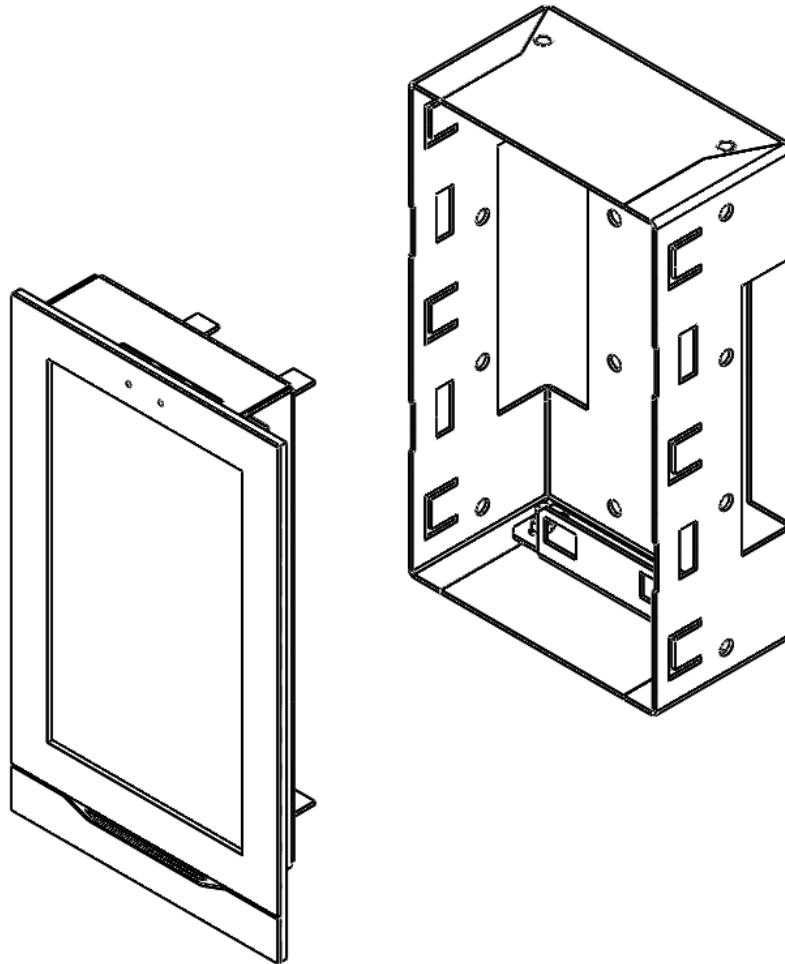
Fig. 2 : Mounting
