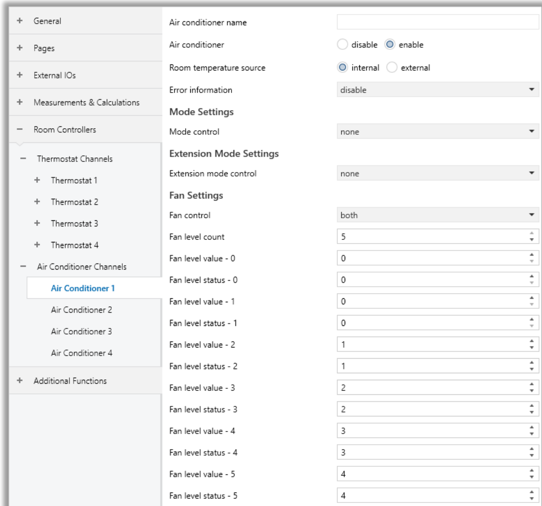
Fig. 70: Air Conditioner – Fan Settings Configuration Page
