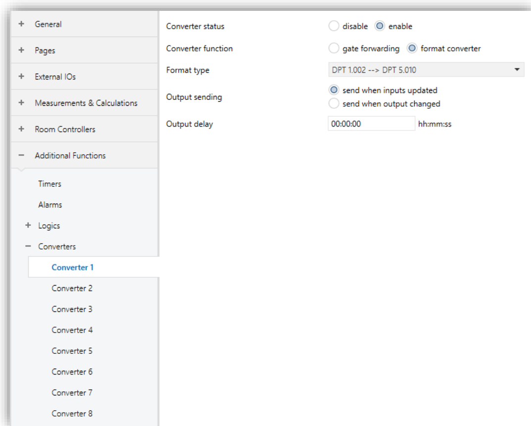
Fig. 82: Logics – Format Converter Configuration
