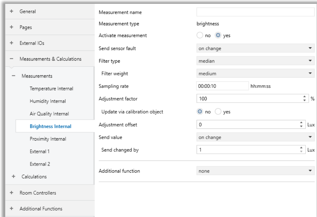
Fig. 35: Brightness Internal Page
