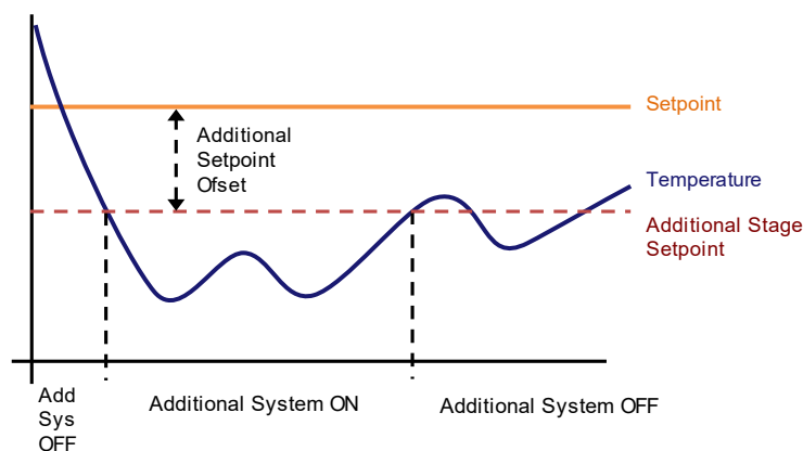
Fig. 50: PI Continuous Graph for Additional Heating Control
