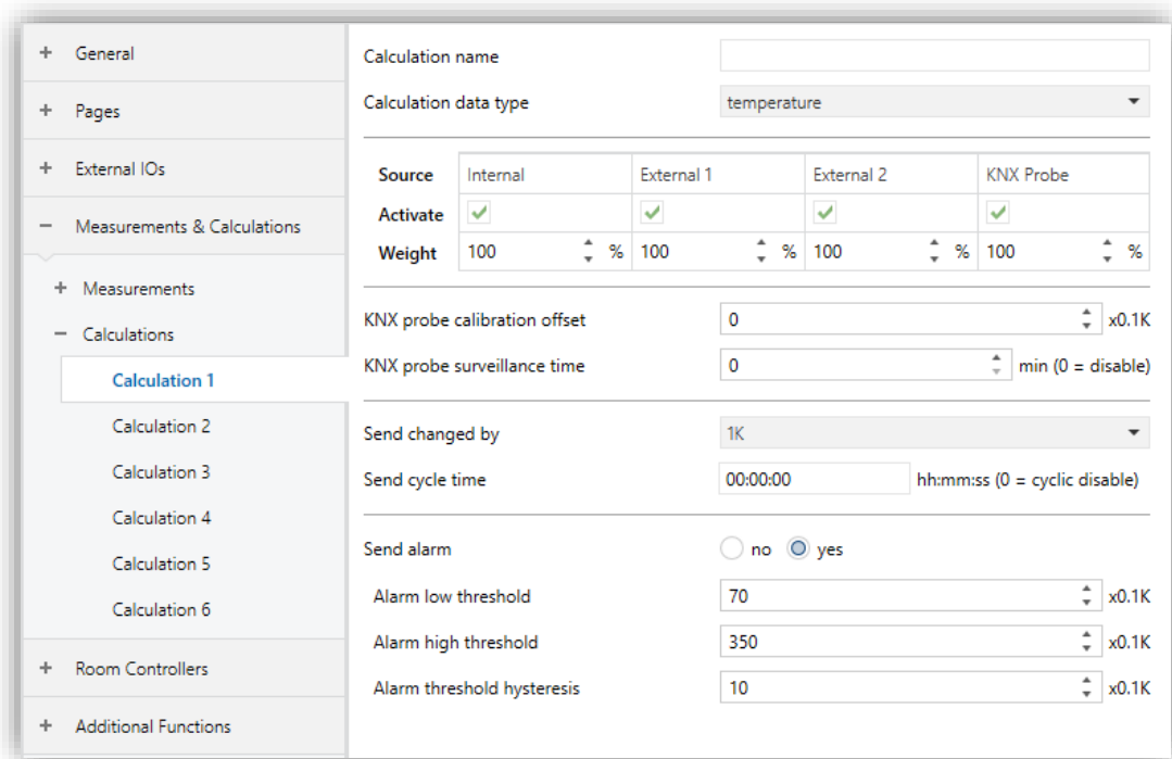
Fig. 39: Calculation for Temperature Page
