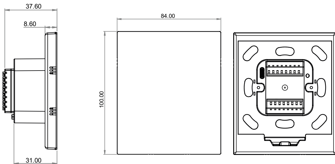
Fig. 1: Dimensions of the iX4
