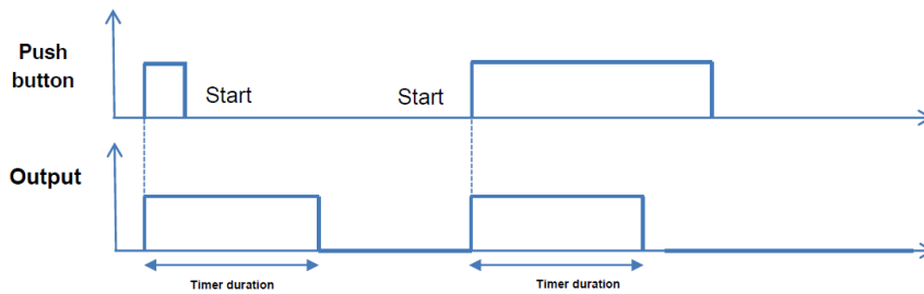
Fig 16 : Timer Operation Behaviour
