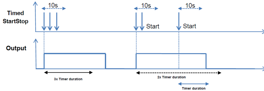
Fig 18 : Timer Retriggerability
