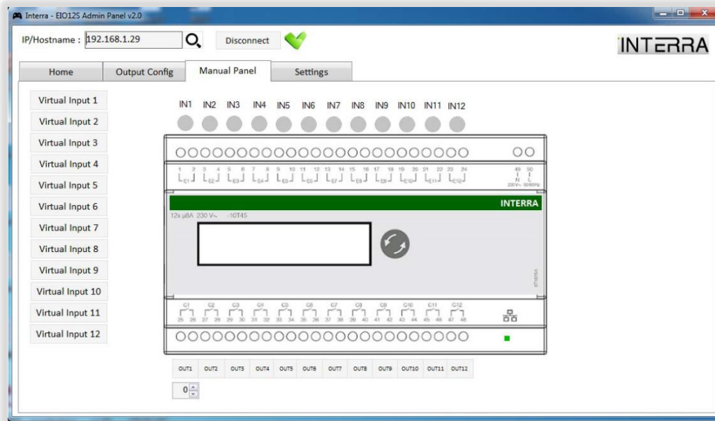
Fig 7 : EIO Configuration Software Manual Panel
