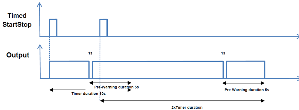
Fig 19 : Timer Retriggerability with Pre-Warning
