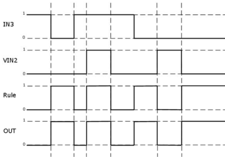
Fig 10 : A Logic Rule Example
