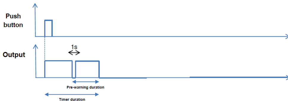
Fig 17 : Pre Warning Behaviour
